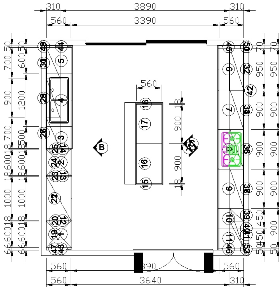
Plan drawing
